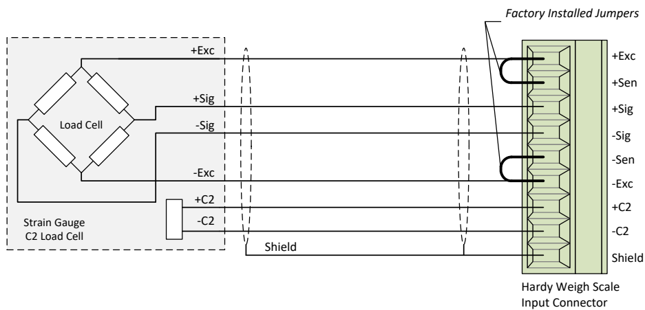
Hardy load sensor with C2 wiring
